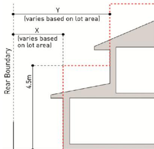
Section showing the minimum rear setback requirements
