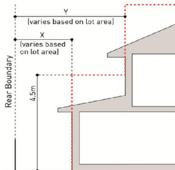
Section showing the minimum rear setback requirements
